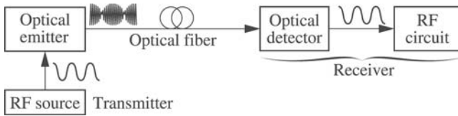
Figure 4.17. Schematic diagram of an optical transmission system with an analog transported signal
