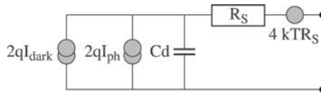
Figure 7.6. Equivalent noise circuit for a reverse-biased PIN photodiode under illumination
