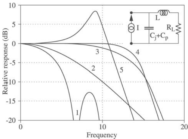
Figure 2.14. Frequency response of a PIN photodiode made of GaInAs/InP at 1.3μm, inserted into the circuit shown. The parameters of each curve are given in Table 2.1
