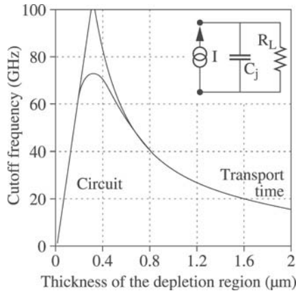
Figure 2.13. 3 dB cutoff frequency of a PIN photodiode, as a function of the thickness of the depleted region. The material is assumed to be GaInAs/InP, the width of the active region 10\mu\text{m} and the load resistance 50\ \Omega
