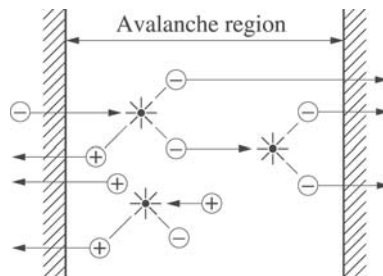
Figure 3.1. Diagram showing the principles of the shock ionization mechanism
