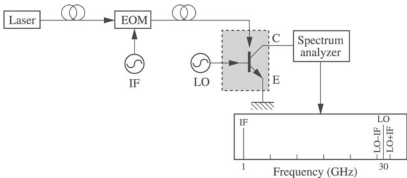
Figure 4.21. Experimental setup for up-conversion from the intermediate frequency IF to a band at 30 GHz, using the HPT as an O/E mixer
