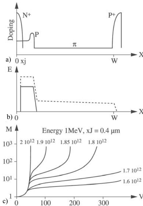
Figure 3.10. Operation principles for a Si N + \pi P \pi P + APD: a) doping profile, b) typical electric field, c) typical M(V) characteristics for different implantation doses of Boron (in \text{cm}^{-2} )
