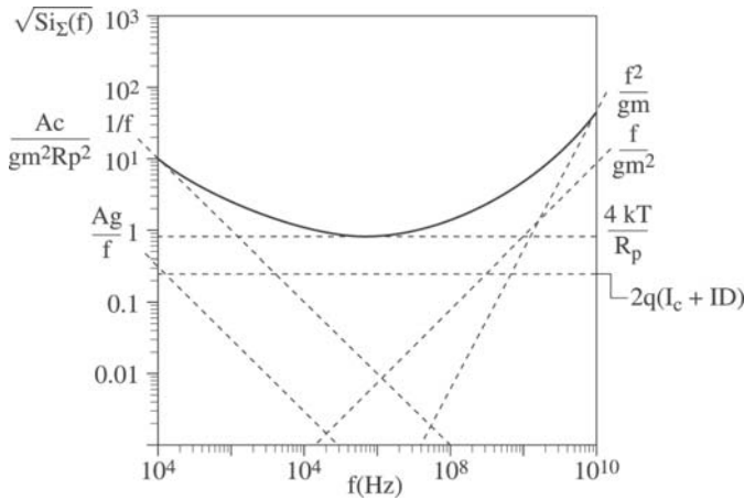
Figure 7.17. Calculation of \sqrt{S_{i_\Sigma}(f)} as a function of frequency, using the appropriate values for the characteristic parameters of the photoreceiver. Dotted lines indicate the contributions from 1/f noise, thermal and shot noise, as well as those of the f and f^2 contributions
