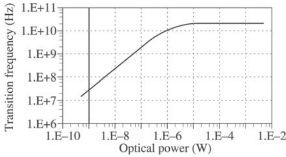
Figure 4.7. Variation in transition frequency f_{TO} with incident optical power P_{opt} . At weak P_{opt} , f_{TO} varies rapidly up to a certain limiting value of P_{opt} , after which it remains constant
